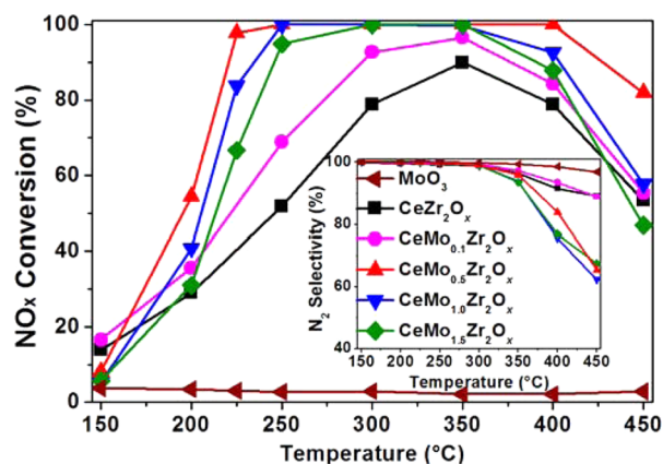
Figure 1. NO x conversion and N 2 selectivity (inserted) in the NH 3 -SCR reaction as a function of the temperature over pure MoO 3 and CeMo a Zr 2 O x ( a = 0, 0.1, 0.5, 1.0, 1.5 ) catalysts. Reaction conditions: [NO] = [NH 3 ] = 500 ppm, [O 2 ] = 5 vol %, and GHSV = 50000 h -1 .
