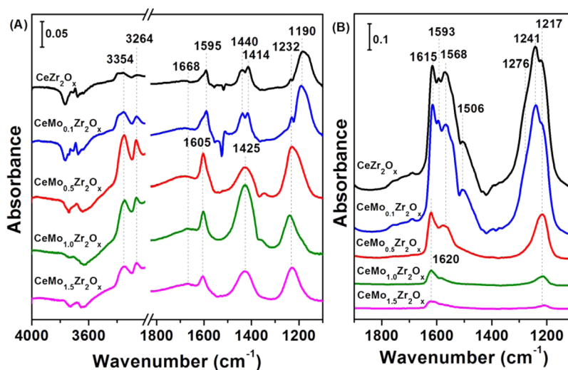
Figure 9. In situ DRIFTS of \text{NH}_3 adsorption (A) and \text{NO} + \text{O}_2 adsorption (B) at 200\text{ }^\circ\text{C} on the \text{CeMo}_x\text{Zr}_2\text{O}_x series of catalysts.
